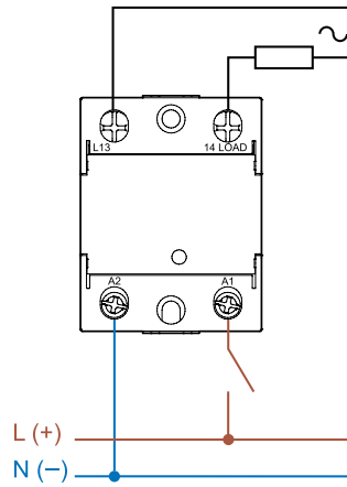
Single-phase connection (77.x1)
