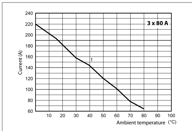
L77-24 Output RMS current v ambient temperature 77.F3.x.xxx.8671
